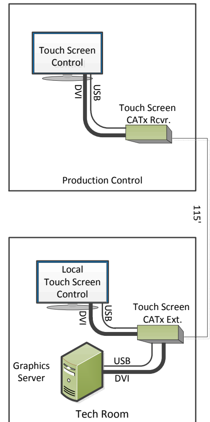
Example 3 Extend Touch Screen control to remote Touch Screen monitor
